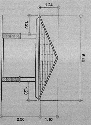
REAR ELEVATION SCALE: 1:50 MTS.
