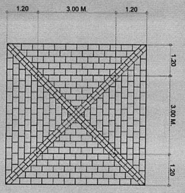
ROOF PLAN OF GAZEBO SCALE: 1:50 MTS.
