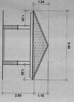
LEFT SIDE ELEVATION SCALE: 1:50 MTS.
