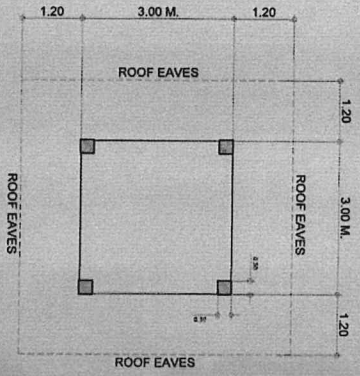
FLOOR PLAN OF GAZEBO SCALE: 1:50 MTS.
